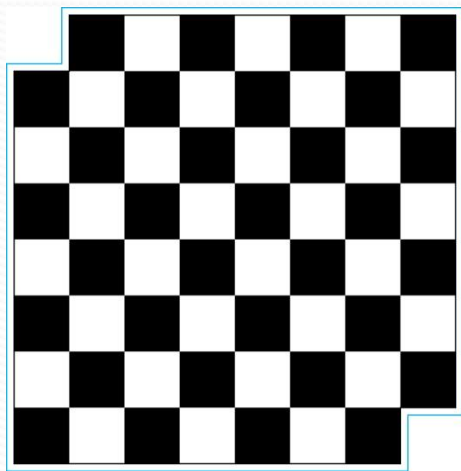
Nonstandard Checkerboard
